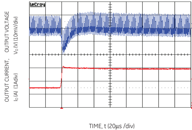
Figure 16. Transient Response to Dynamic Load Change from 50% to 100% at 12Vin, C_{out}=1\times 47\mu\text{F}+1\times 330\mu\text{F} , C_{Tune}=10\text{nF} & RTune=261
