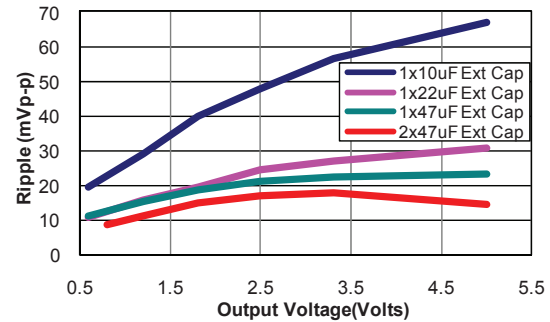
Figure 38. Output ripple voltage for various output voltages with external 1x10 \mu F, 1x22 \mu F, 1x47 \mu F and 2x47 \mu F ceramic capacitors at the output (3A load). Input voltage is 12V.
