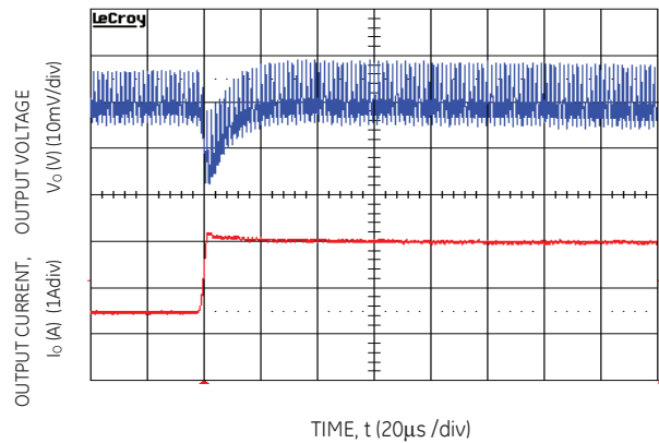
Figure 10. Transient Response to Dynamic Load Change from 50% to 100% at 12V in , C out -1x47μF+1x330μF, C Tune -10nF & R Tune -261
