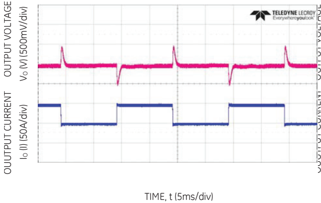
Figure 7. Transient response 12V DC output load step 10 – 60A, V IN = -48V DC .
