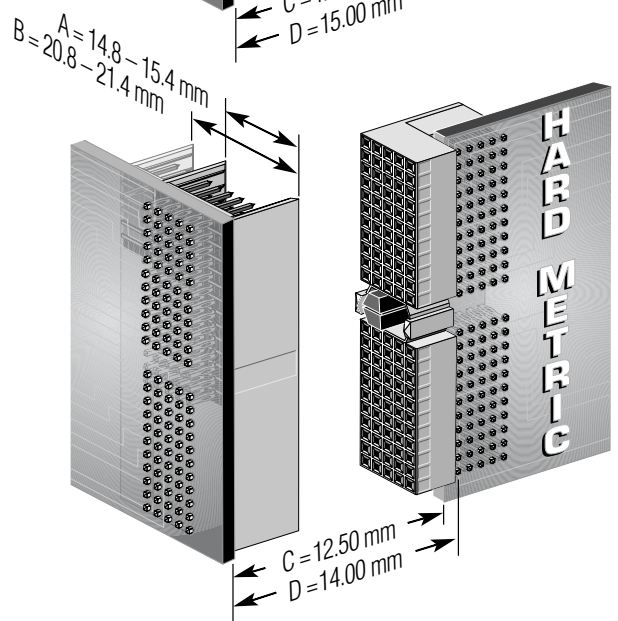
ERmet 2mm H.M. Connectors
