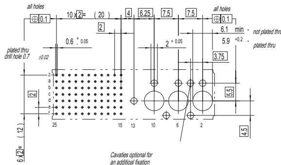
Board hole pattern (Component mounting side) for press-fitting
