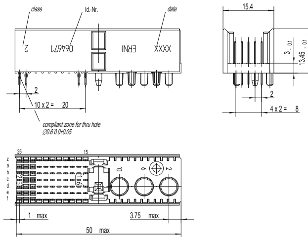
Board hole pattern (Component mounting side)
