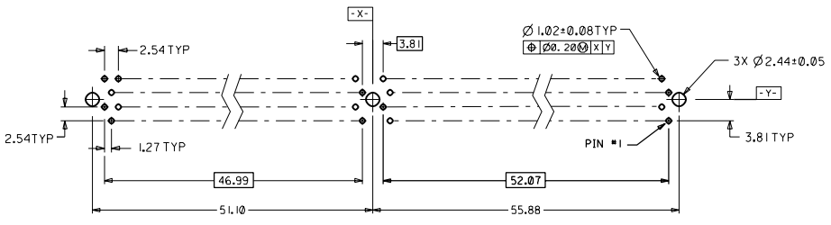
RECOMMENDED MATING P.C BOARD CONFIGURATION
