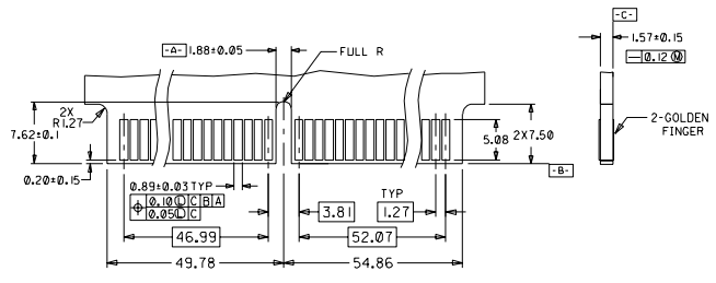
RECOMMENDED MATING PCB EDGE CONFIGURATION
