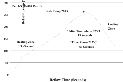
Figure 51. Recommended linear reflow profile using Sn/Ag/Cu solder.
