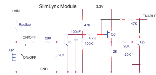
Figure 40. Circuit configuration for using negative On/Off logic.
