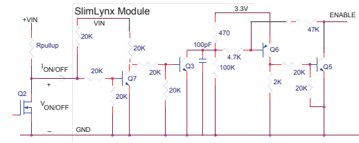
Figure 39. Circuit configuration for using positive On/Off logic.
