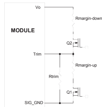
Figure 43. Circuit Configuration for margining Output voltage.
