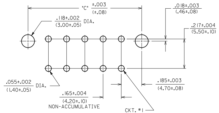
RECOMMENDED HOLE LAYOUT FOR .070/(1.78) MAX. THICK P. C. BOARD SHOWN FROM COMPONENT SIDE
