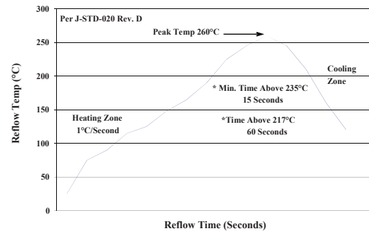
Figure 48. Recommended linear reflow profile using Sn/Ag/Cu solder.
