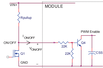
PVX012 NEGATIVE LOGIC FIGURE
