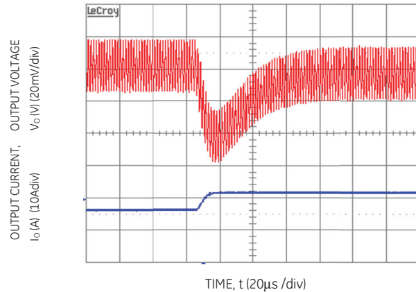
Figure 22. Transient Response to Dynamic Load Change from 50% to 100% at 12Vin, C_{out}=1\times 47\mu F+1\times 330\mu F , C_{Tune}=3300pF & R_{Tune}=270ohms
