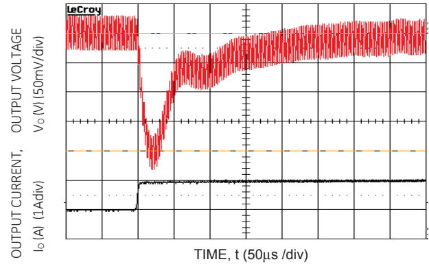
Figure 16. Transient Response to Dynamic Load Change from 50% to 100% at 28Vin, C_{ext} = 3 \times 10\mu F ceramic, C_{Tune} = 47pF & R_{Tune} = 332\Omega
