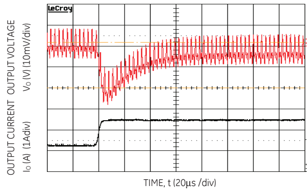
Figure 4. Transient Response to Dynamic Load Change from 50% to 100% at 28Vin, C_{ext} = 10\mu F ceramic + 330uF polymer, C_{Tune} = 5600pF & R_{Tune} = 261\Omega
