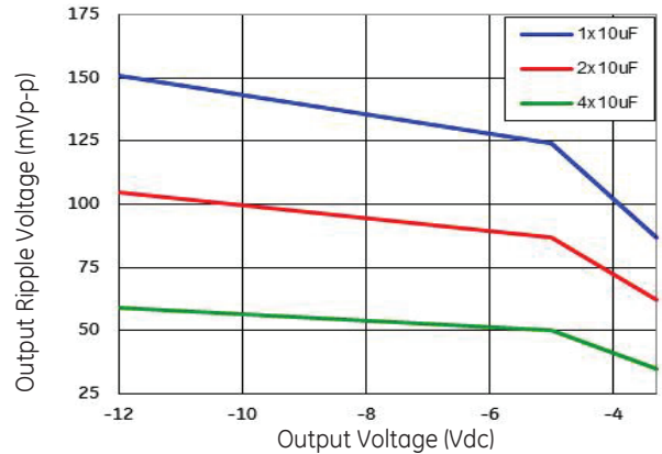
Figure 64. Output ripple with 1x10µF, 2x10µF & 4x10µF output ceramic capacitors (max load).
