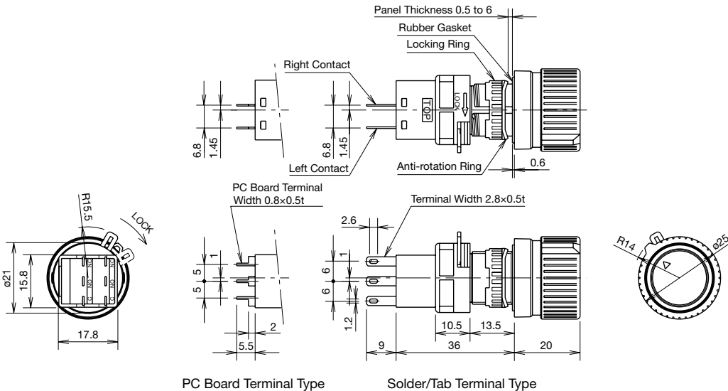
PC Board Terminal Type
