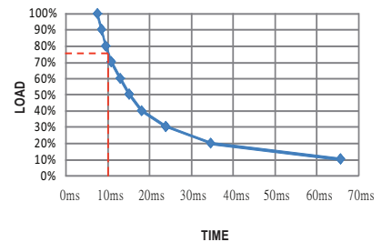
RSD-150C-24
