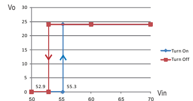
RSD-150D-24
