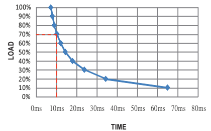
RSD-150C-24
