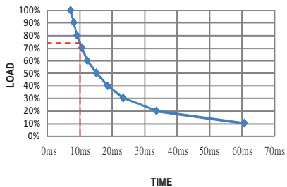
RSD-150C-5
