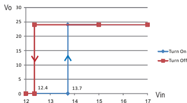
RSD-150B-24
