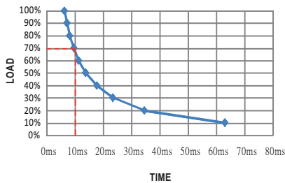
RSD-150C-5
