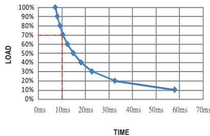
RSD-150C-12
