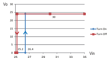
RSD-150C-24
