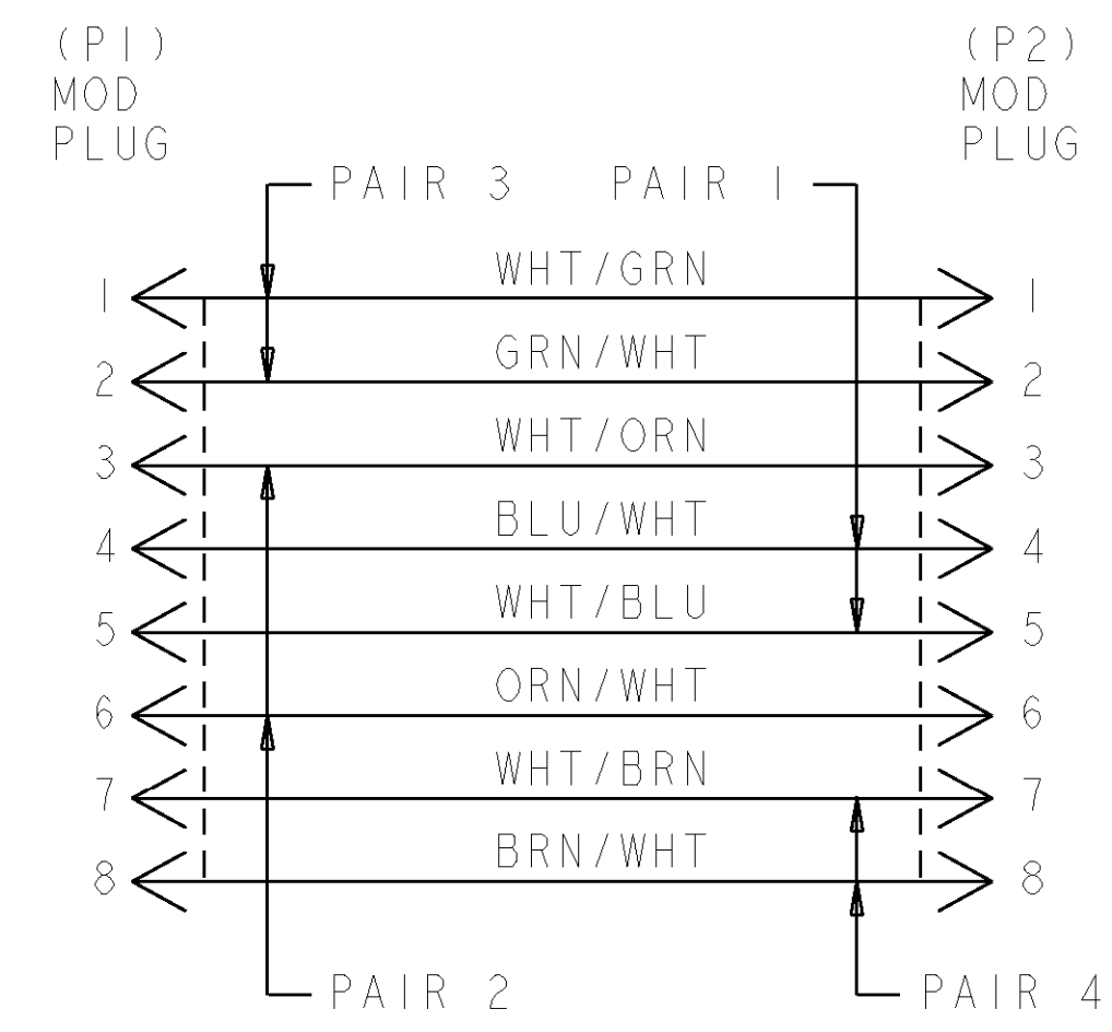
WIRING DIAGRAM 568A
