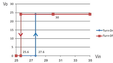
RSD-100C-24
