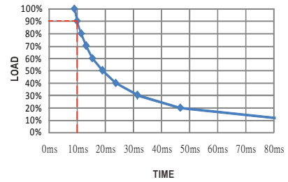
RSD-100C-24
