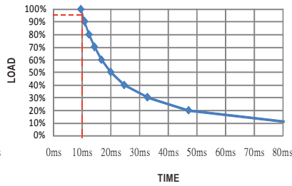
RSD-100C-12
