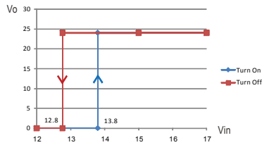
RSD-100B-24
