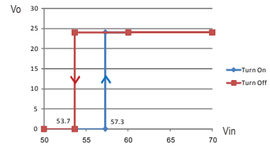
RSD-100D-24
