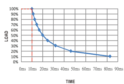
RSD-100C-24
