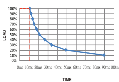
RSD-100C-5
