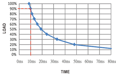
RSD-100C-5
