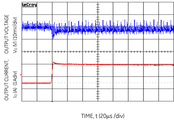
Figure 4. Transient Response to Dynamic Load Change from 50% to 100% at 8Vin, C out -1x47µF+2x330µF, C Tune -27nF, R Tune -178
