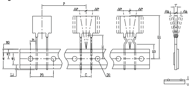
Figure 2 - PTR030V0500-PTR030V0900
