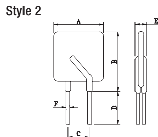
Figure 1 - PTR030V0090-PTR030V0400
