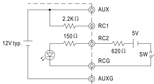
(A) Using external voltage source
