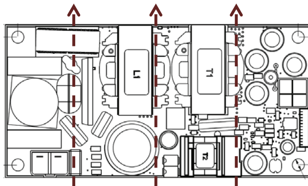
Fig. 11. Preferred airflow direction for cooling.
