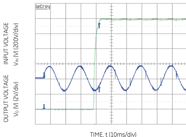
Figure 5. Typical Start-up ( V_{IN} = 115\text{Vac} ).
