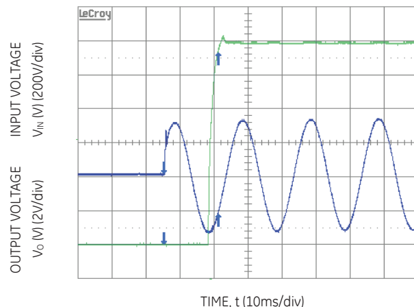
Figure 6. Typical Start-up ( V_{IN} = 230\text{Vac} ).
