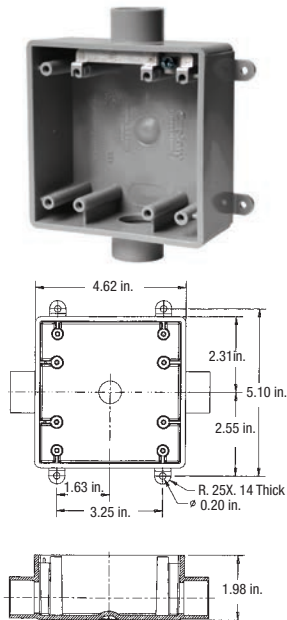
Type 2FSC
