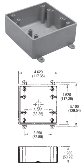
Type FS
