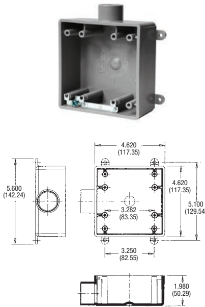
Type 2FSE
