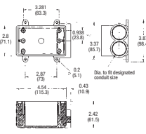
Type FSS
