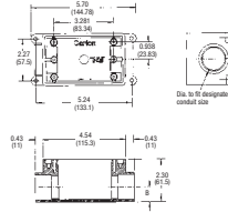
Type FSC
