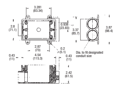
Type FSCC
