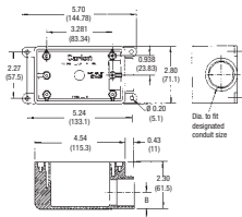
Type FSE
