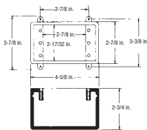
Type FD
