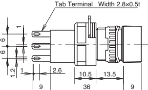
Solder/Tab Terminal
