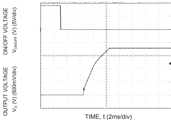
Figure 15. Typical Start-up Using On/Off Voltage ( I_o = I_{o,max} ).
