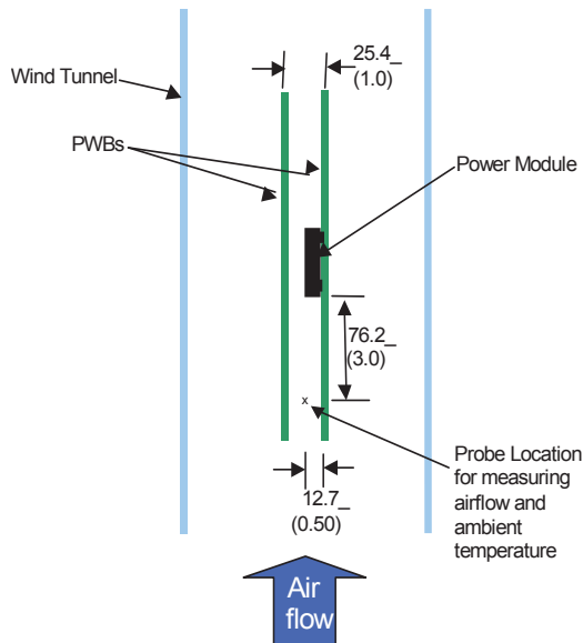
Figure 35. Thermal Test Setup.
