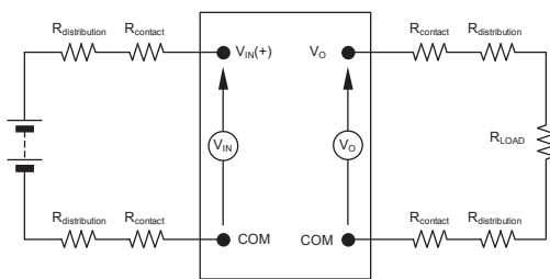
Figure 26. Output Voltage and Noise Test Setup.
