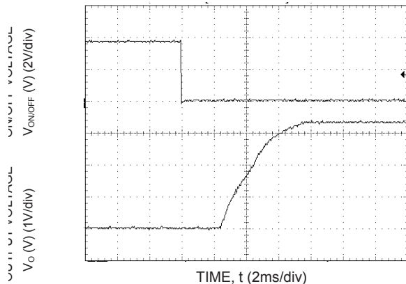
Figure 21. Typical Start-up Using On/Off Voltage ( I_o = I_{o,max} ).
