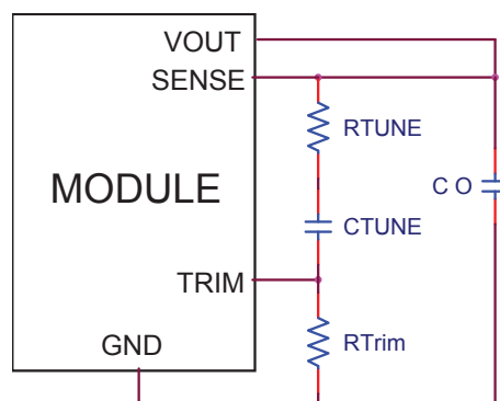
Figure 34. Circuit diagram showing connection of R_{TUNE} and C_{TUNE} to tune the control loop of the module.
