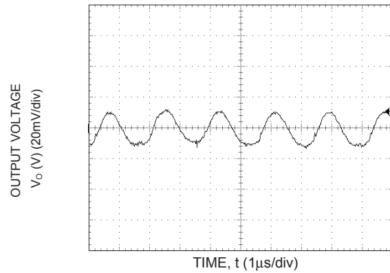
Figure 2. Typical output ripple and noise ( V_{IN} = 12V , I_O = 30A , C_{OUT} = 0.1\mu F \parallel 47\mu F ceramic capacitors).
