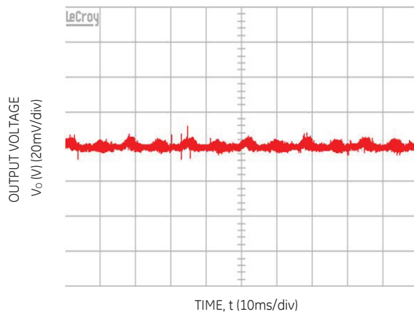
Figure 6. 5V DC output ripple and noise, all full load, V_{IN} = 185V_{AC} .
